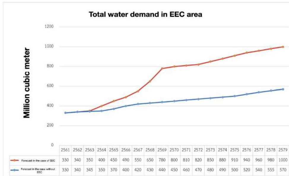
Figure 1: Water volume and forecast of total water demand within the Eastern Economic Corridor (The Royal Irrigation Department, 2020)
